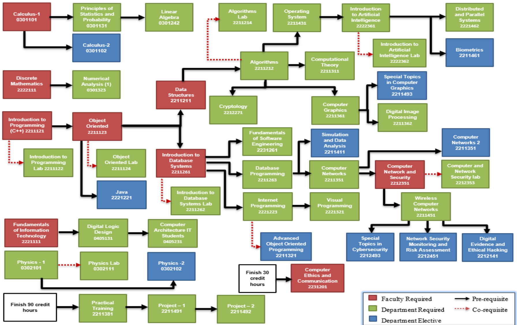
Figure 5-1. Curriculum Bachelor of Information Technology in Computer Information System.
